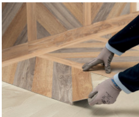
Installation of MODULAR LVT with Ultrabond Eco V4 Evolution
